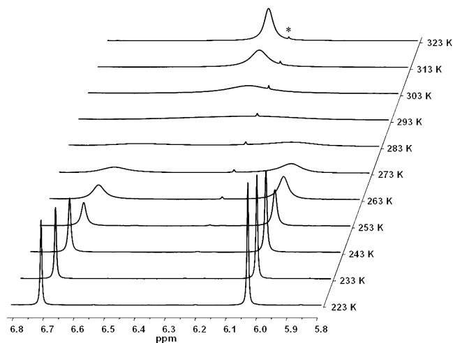
Fig. 3 VT ^1\text{H} NMR (500 MHz) spectra of 7\beta in \text{CDCl}_3 between 6.8–5.8 ppm for temperatures 223 K to 323 K. * Trace impurity.
