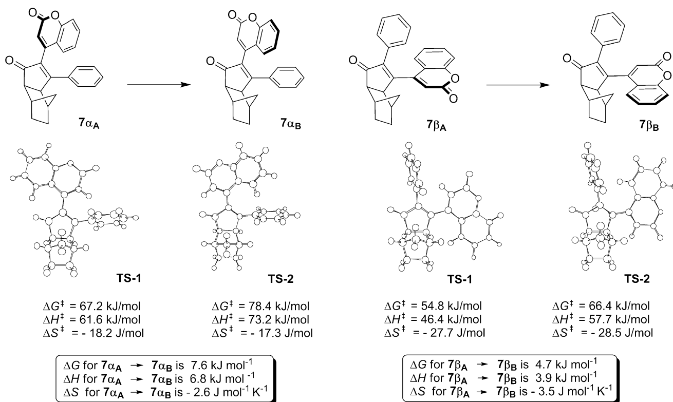
Fig. 6 Theoretically determined energetic parameters for both of the regioisomeric products 7\alpha and 7\beta . For each process, two different transition state structures were calculated considering the clockwise and anticlockwise rotations about the single C–C bond connecting the coumarin moiety to the cyclopentenone framework.
